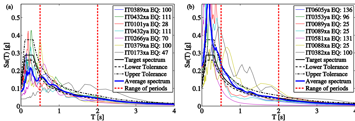
Figure 5. Record selection for Terni and T_r=475 yr considering spectrum compatibility and PGV values derived from 1 st and 2 nd modal values of disaggregation.
